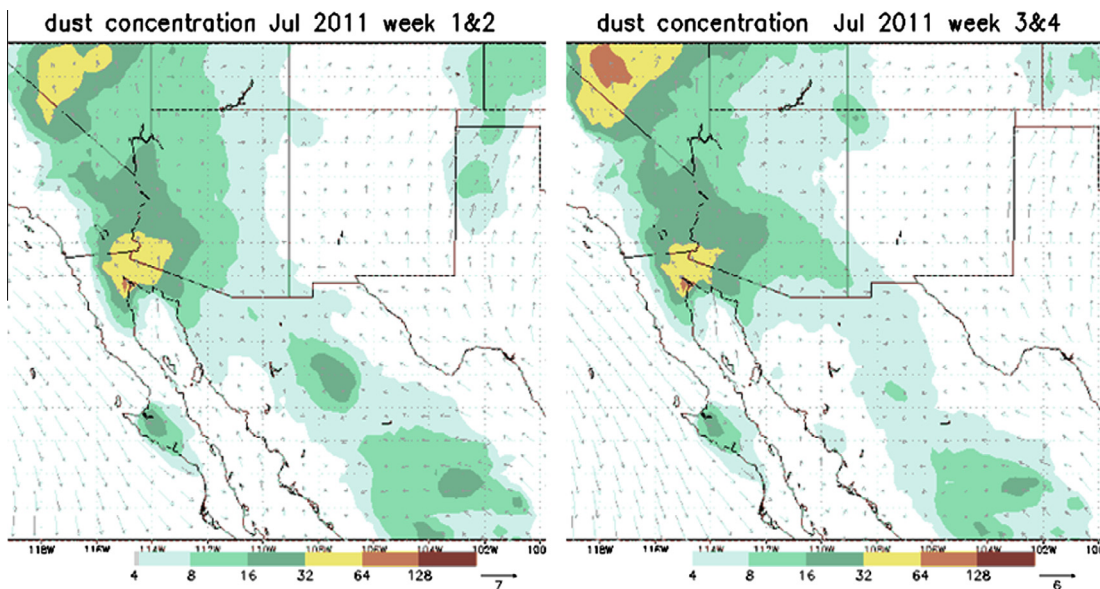
Fig. 16a. Model hindcast of surface dust concentrations ( \mu\text{g m}^{-3} ) averaged over (L) the first two weeks and (R) the last two weeks of July 2011.
