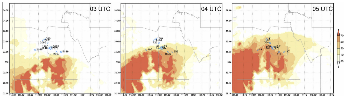
Fig. 9. NMME-DREAM PM_{10} ( \mu g m^{-3} ) surface dust concentration (orange) and observed (blue dots) values of PM_{10} ( \mu g m^{-3} ) at 03, 04 and 05 UTC on 6 July 2011 for Maricopa County, Arizona (from Vukovic et al., 2014). (For interpretation of the references to colour in this figure legend, the reader is referred to the web version of this article.)
