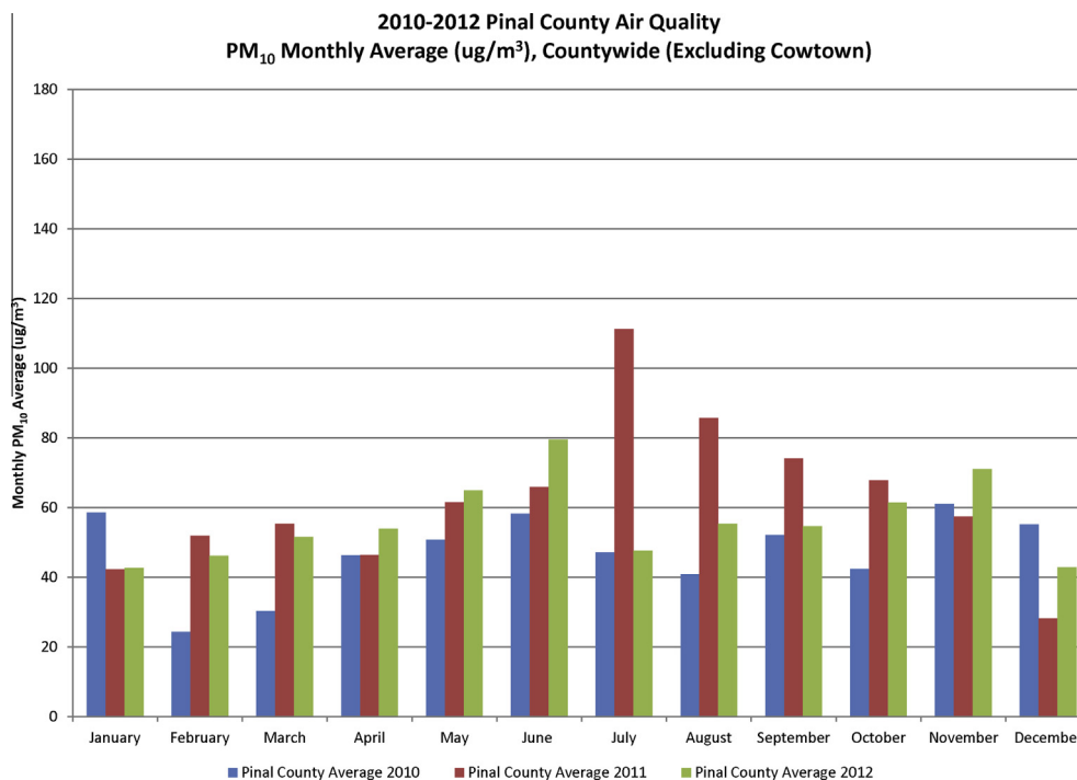
Fig. 11. 2010–2012 Pinal County Air Quality PM 10 Monthly Average (μg m -3 ), Countywide from 5 continuous monitoring stations.
