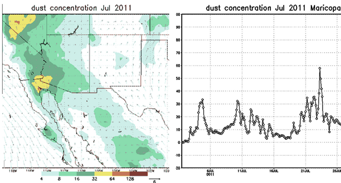
Fig. 16b. Model hindcast of surface dust concentrations ( \mu\text{g m}^{-3} ) (L) averaged over the month of July 2011 and (R) the July 2011 evolution of dust concentration ( \mu\text{g m}^{-3} ) in Maricopa County, Arizona.
