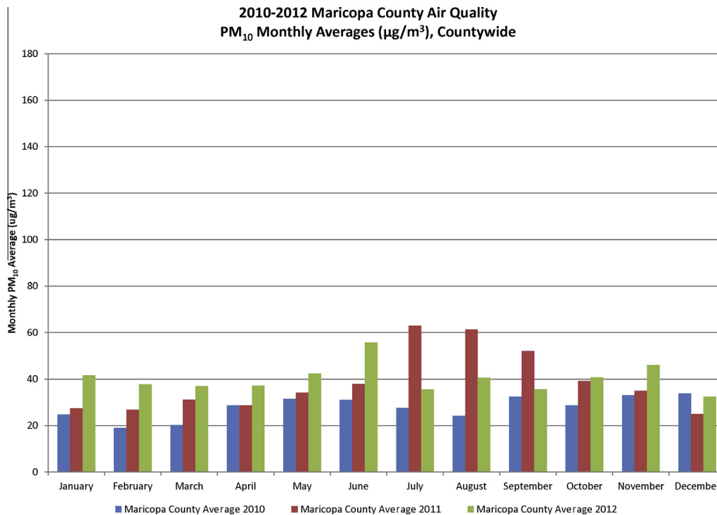
Fig. 10. 2010–2012 Maricopa County Air Quality PM 10 Monthly Average ( \mu\text{g m}^{-3} ), Countywide from 15 continuous monitoring stations.
