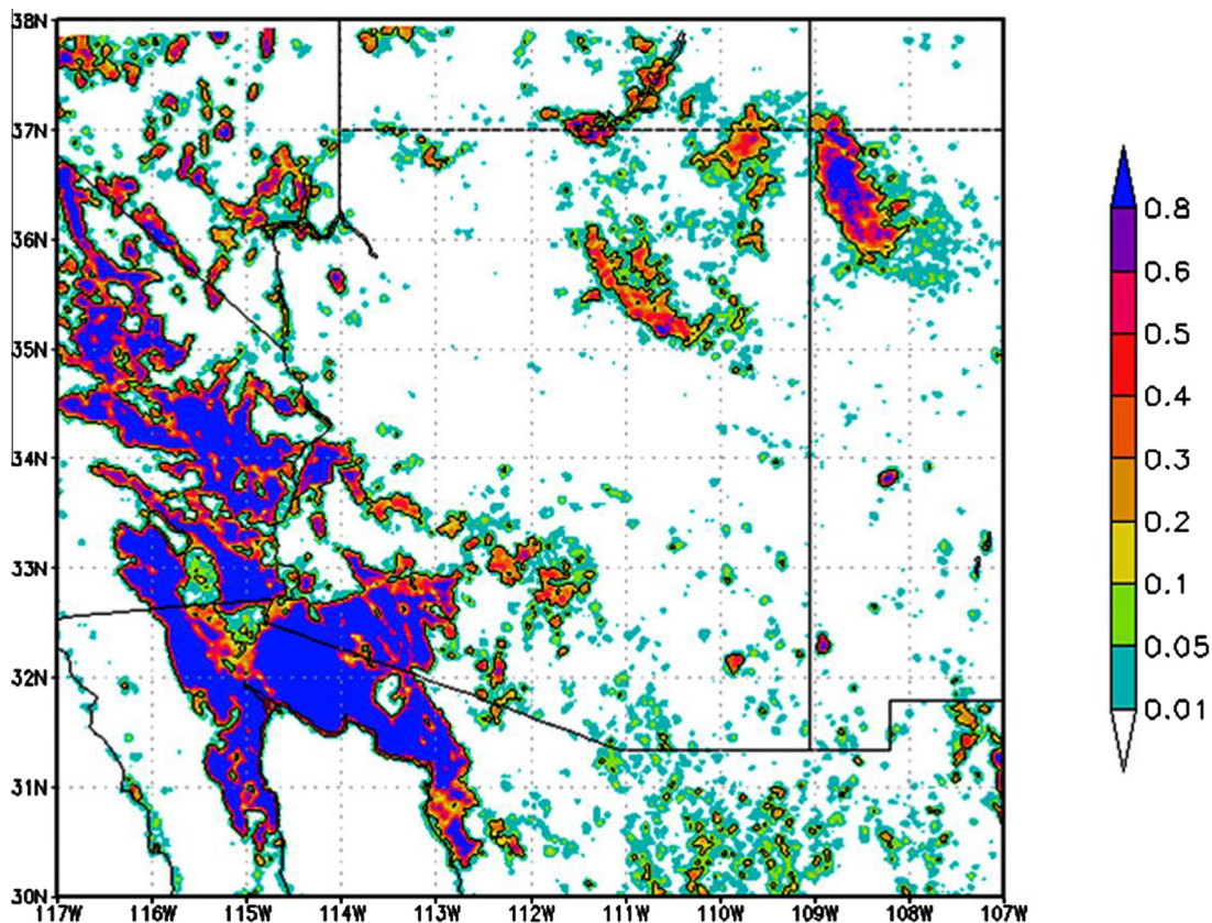
Fig. 8. Potential dust sources are identified from NASA’s Moderate Resolution Imaging Spectroradiometer (MODIS) to create a mask on 3.5 km model resolution. The mask includes barren, sparsely vegetated and farmland areas that are currently without vegetation.
