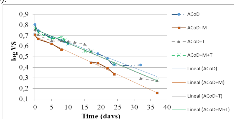
Figure 3. Velocity of the anaerobic reactions in codigestion of agricultural waste in presence of pesticides
