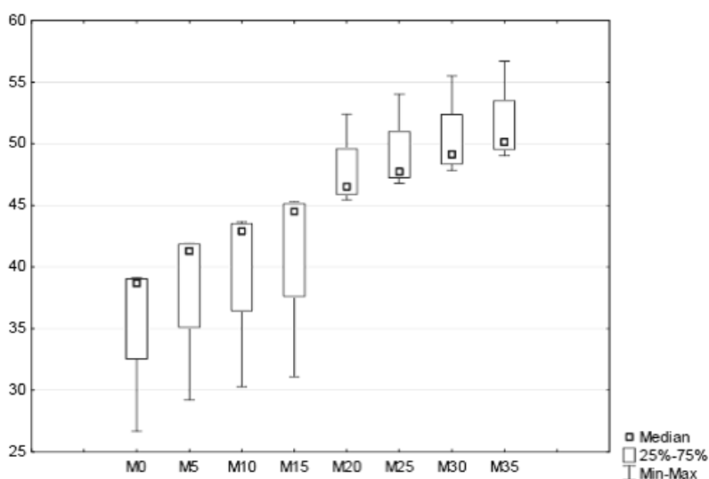
Graph 5: Extracts of dried Rosmarinus officinalis L.
