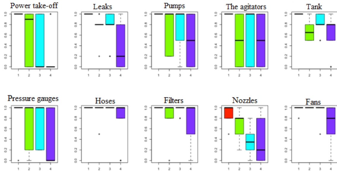
Figure 3 Effect of exploitation period on the tested orchard sprayer elements technical functionality
