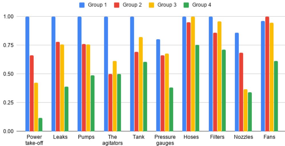
Figure 2 Display of assessment of tested orchard sprayer elements technical functionality by groups
