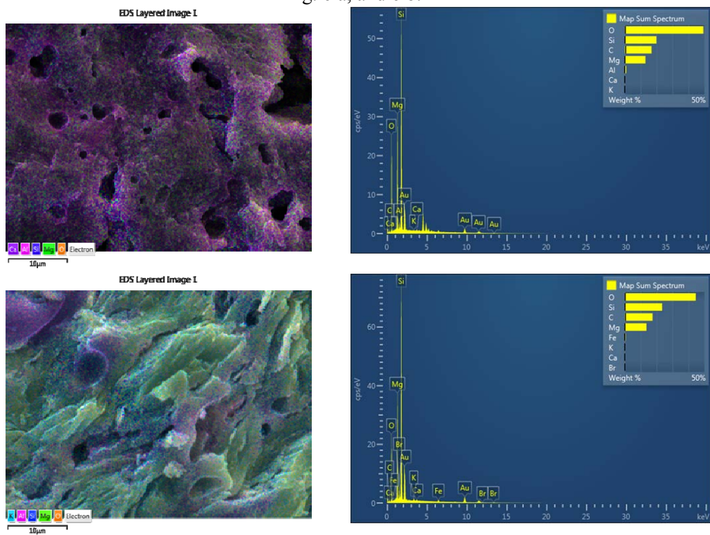
Fig. 9. EDS mapping (left), and elemental analyses (right) of the steatite samples from Fig. 7 a, and 7 b.
